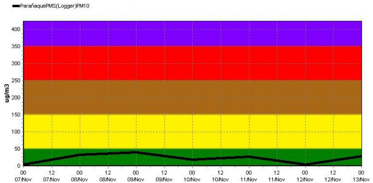
AIR QUALITY MONITORING STATION IN THE ROADSIDE OF THE CITY Period: 11/7/2015 - 11/13/2015 Resolution: 1440 minutes
